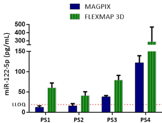
Fig. 3 miR-122-5p quantification with MAGPIX and FLEXMAP 3D platforms. On the x axis is shown the ID for the samples, whereas the y-axis reports the miR-122-5p concentration in \text{pg mL}^{-1} . PS means patient sample; blue columns refer to MAGPIX; green columns refer to FLEXMAP 3D.
