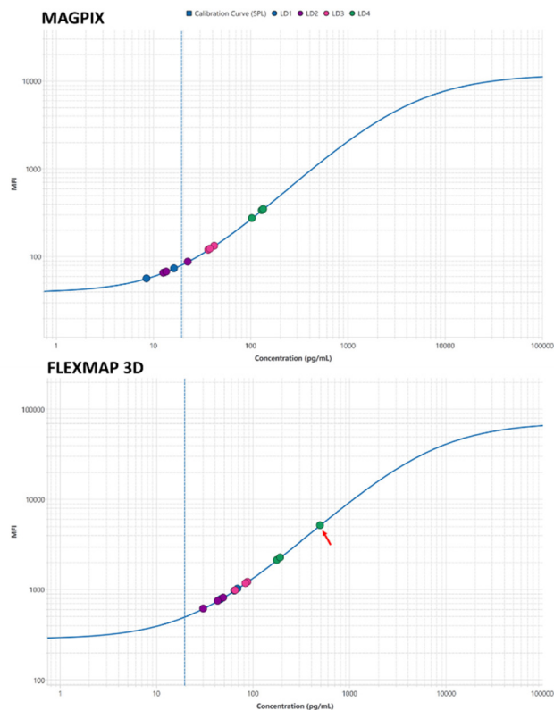
Fig. 2 Calibration curves. Calibration curves were constructed by utilising a SPL non-linear regression model, where MFI average values were plotted against the concentration of synthetic miRNA-122-5p. The curve generated using the MAGPIX platform for Experiment 2 is depicted above, while the curve generated using the FLEXMAP 3D platform for Experiment 2 is displayed below. To signify the LLOQ, a vertical line is indicated on each curve. Each measurement was conducted in triplicate; PS: patient sample; the red arrow indicates the outlier.
